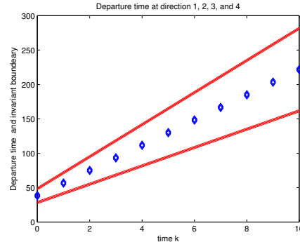
Fig. 2. The traveling time in direction 1, 2, 3, 4.
