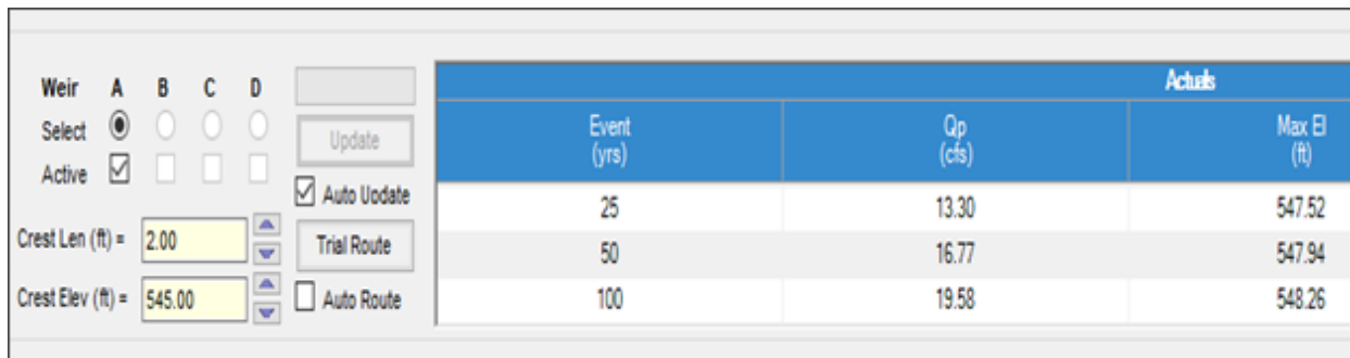
Figure 24: Designing the weir with adjusted the crest length.
