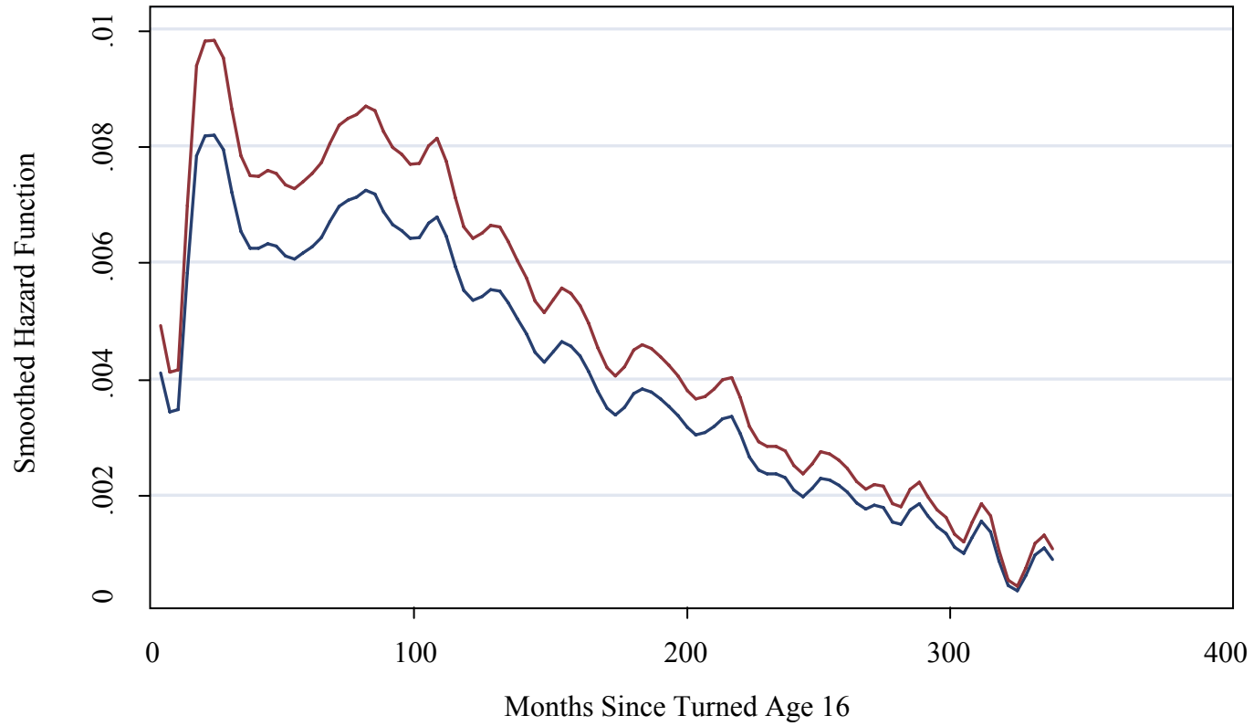
Figure 1 Cox Proportional Hazards Regression
